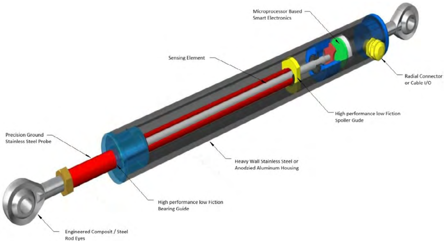
Figure 3 Cutaway View of LVIT
