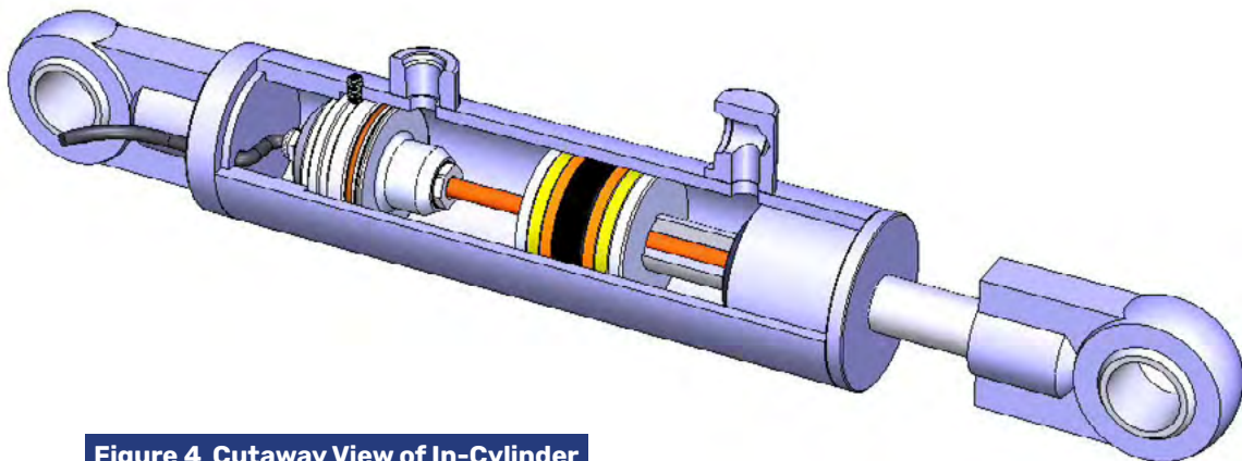
Figure 4 Cutaway View of In-Cylinder
