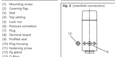
(1) Mounting screw (2) Covering flap (3) Seal (4) Trip setting (5) Lock nut (6) Pressure connection (7) Plug (8) Terminal board (9) Profiled seal (10) Plug housing (11) Fastening screw (12) Pg gland (13) O-Ring
